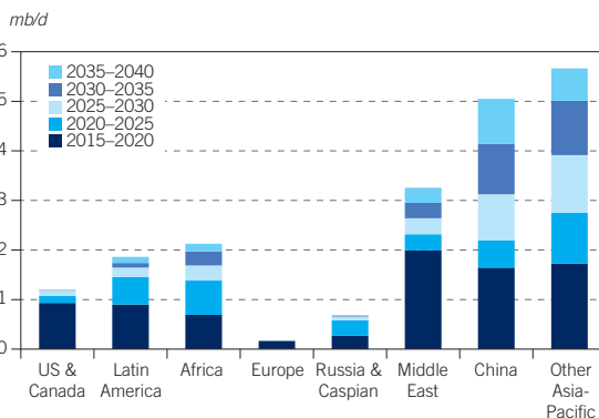
Crude distillation capacity additions in the Reference Case 2015–2040
