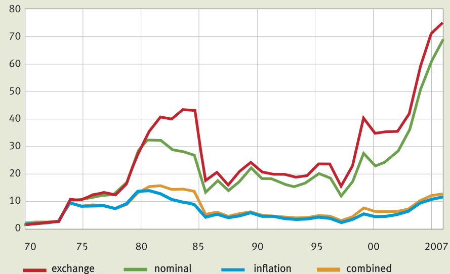
Crude oil prices in nominal and real terms
