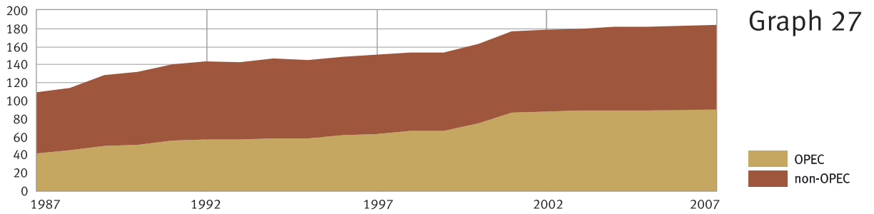
World marketed natural gas production, 1987–2007 (bn cu m)
