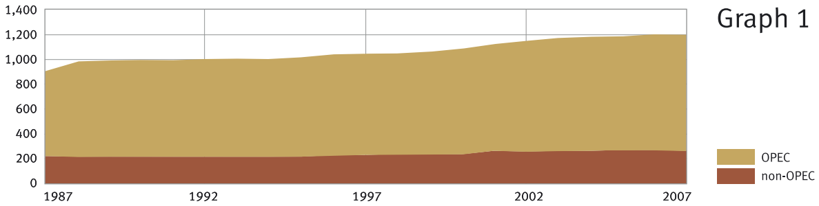
World proven crude oil reserves, 1987–2007 (bn b)
