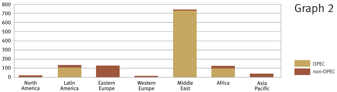
Crude oil reserves by region, 2007 (bn b)
