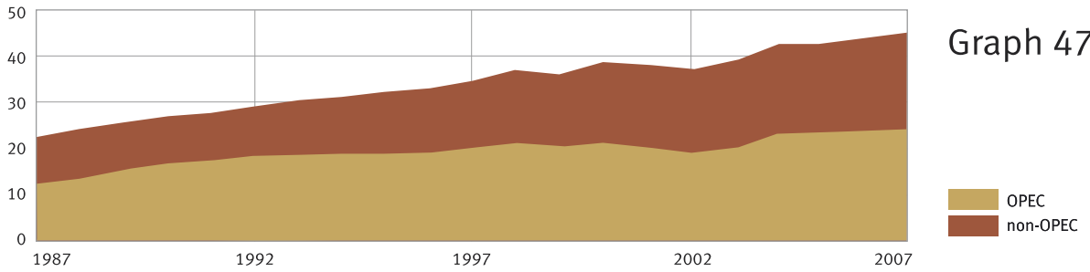
Crude oil exports, 1987–2007 (m b/d)
