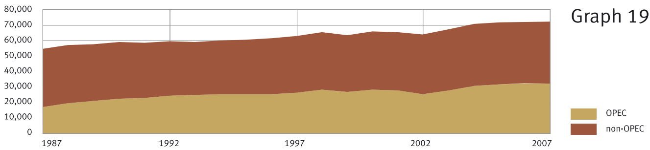
World crude oil production, 1987–2007 (1,000 b/d)
